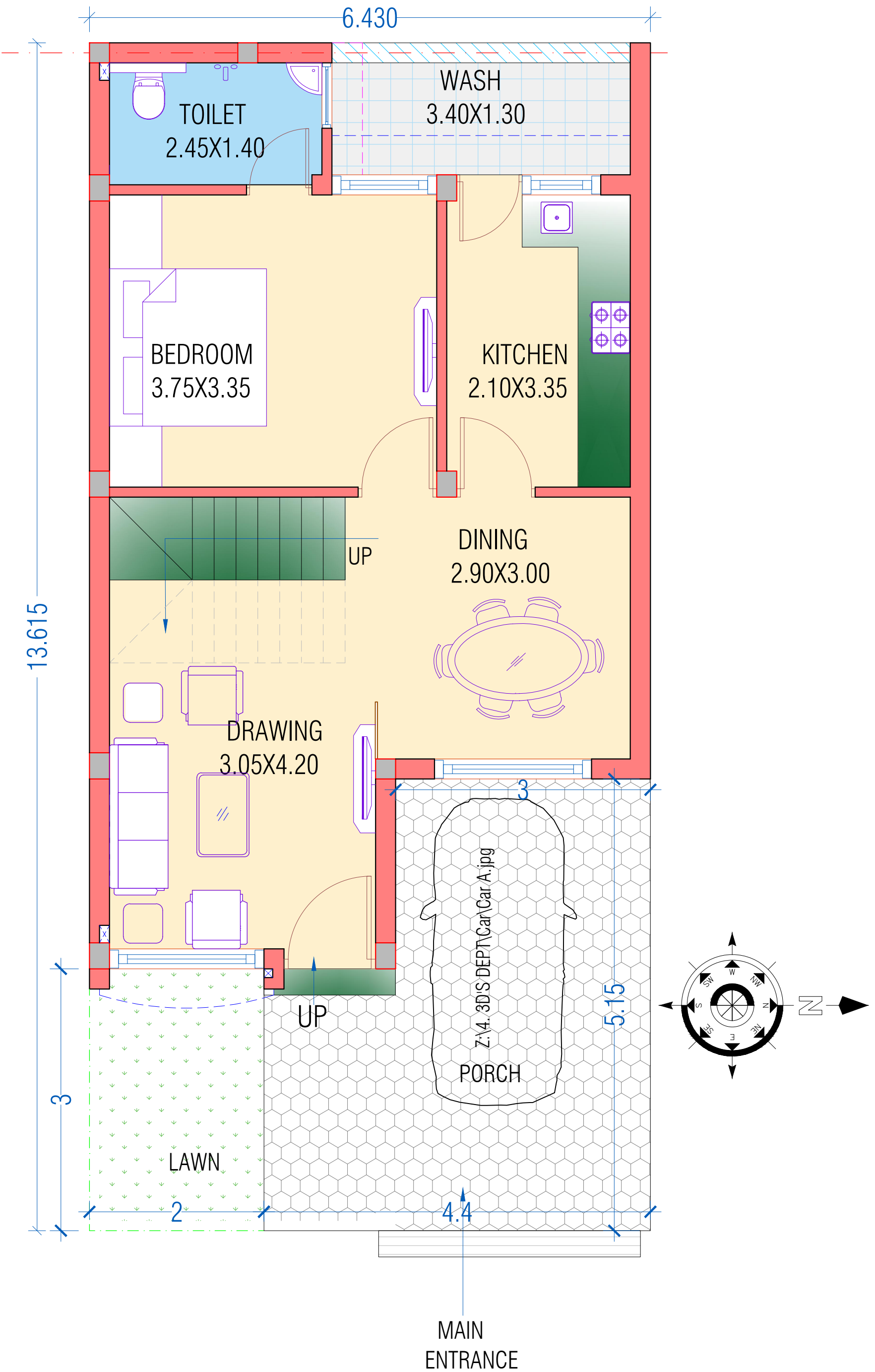
GROUND FLOOR CONCEPT PLAN
